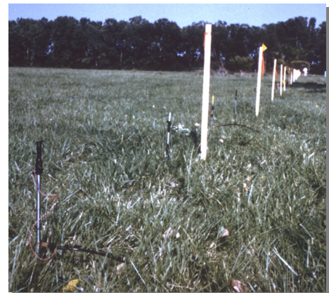
RESISTIVITY ELECTRODES CONNECTED BY MULTICORE CABLE
